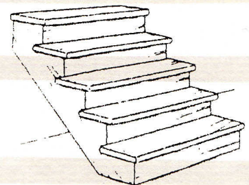
Cut and Mitred String
